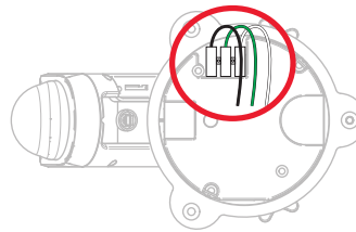
Floodlight camera, bottom 3-wire connector
