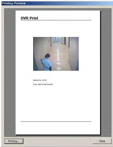
<Preview Window>
